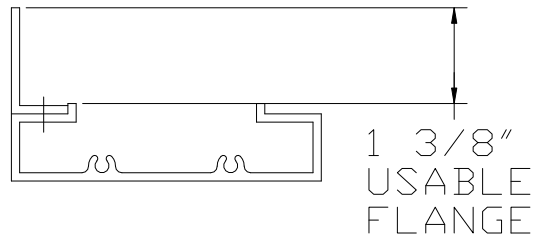
FLANGE FRAME DETAIL
