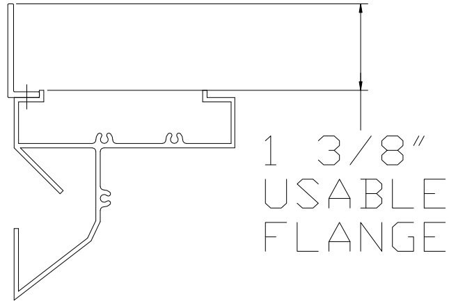
FLANGE FRAME DETAIL
