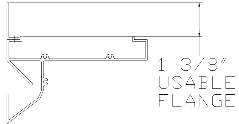
FLANGE FRAME DETAIL
