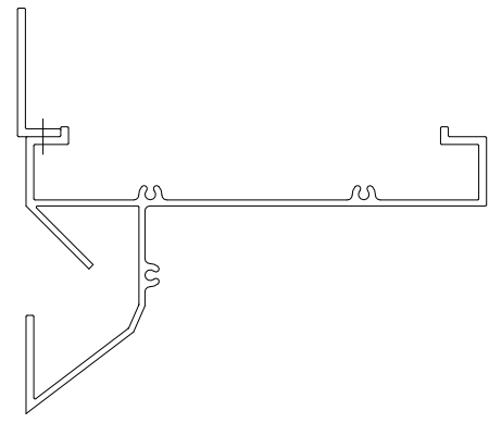
FLANGE FRAME DETAIL
