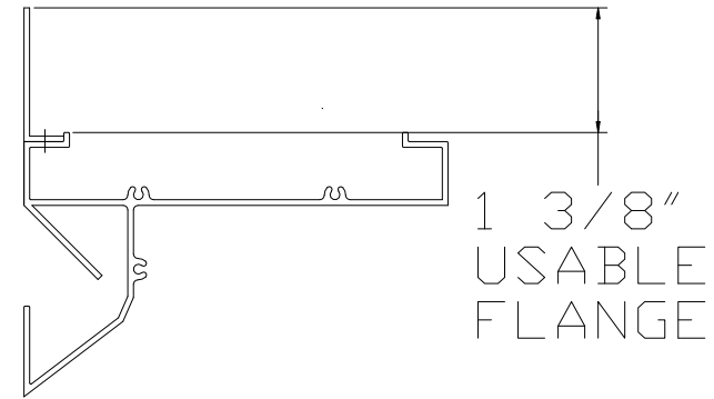
FLANGE FRAME DETAIL
