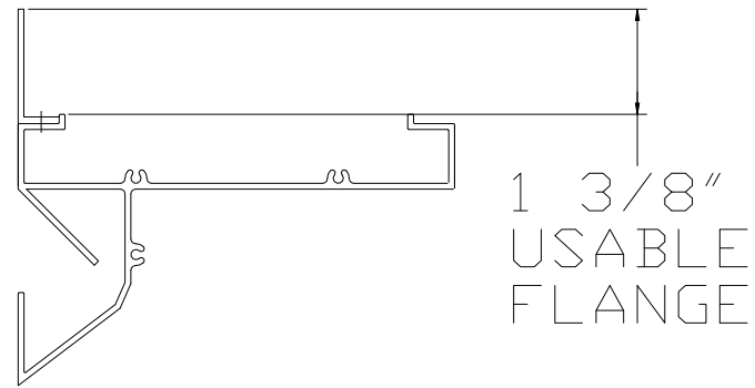
FLANGE FRAME DETAIL
