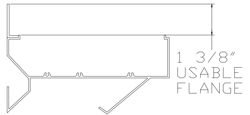
FLANGE FRAME DETAIL
