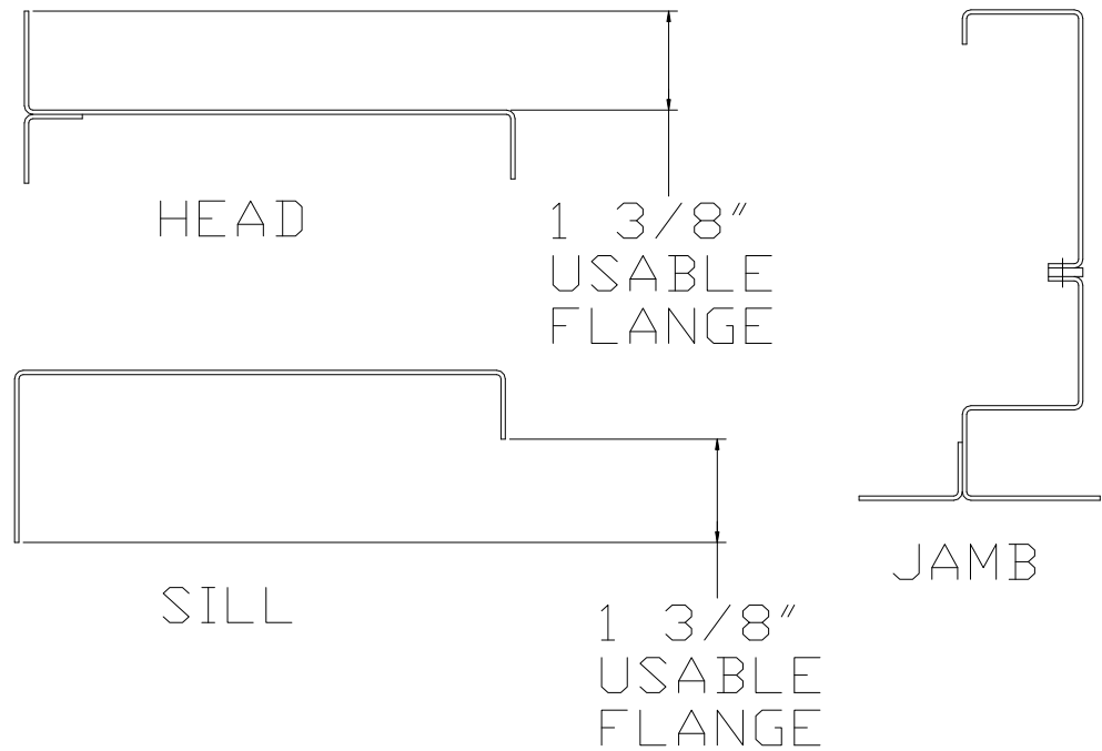
FLANGE FRAME DETAIL
