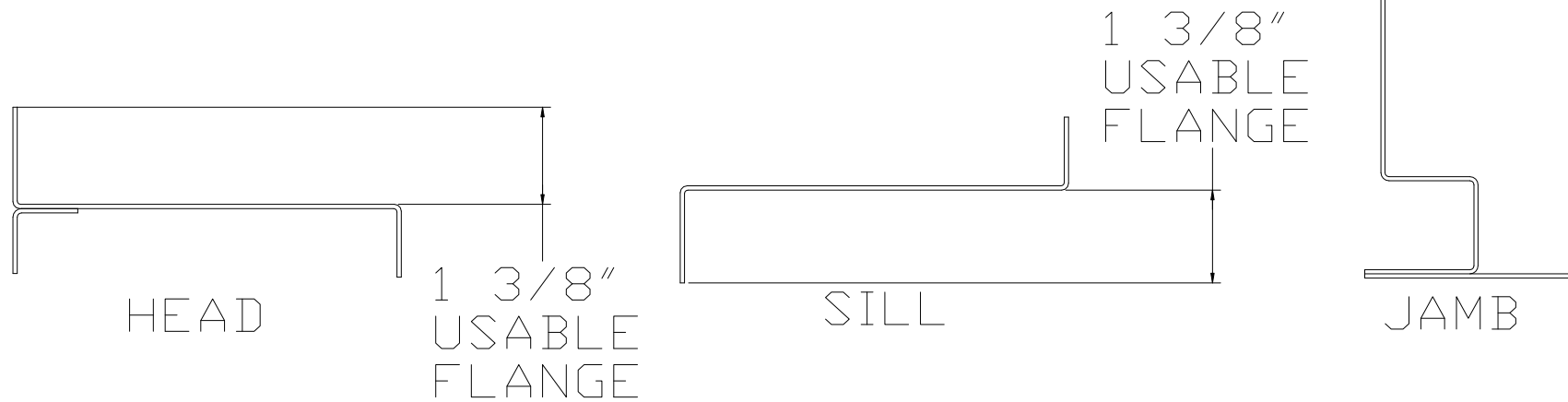
FLANGE FRAME DETAIL
