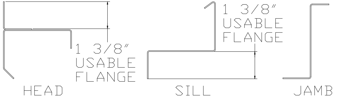
FLANGE FRAME DETAIL
