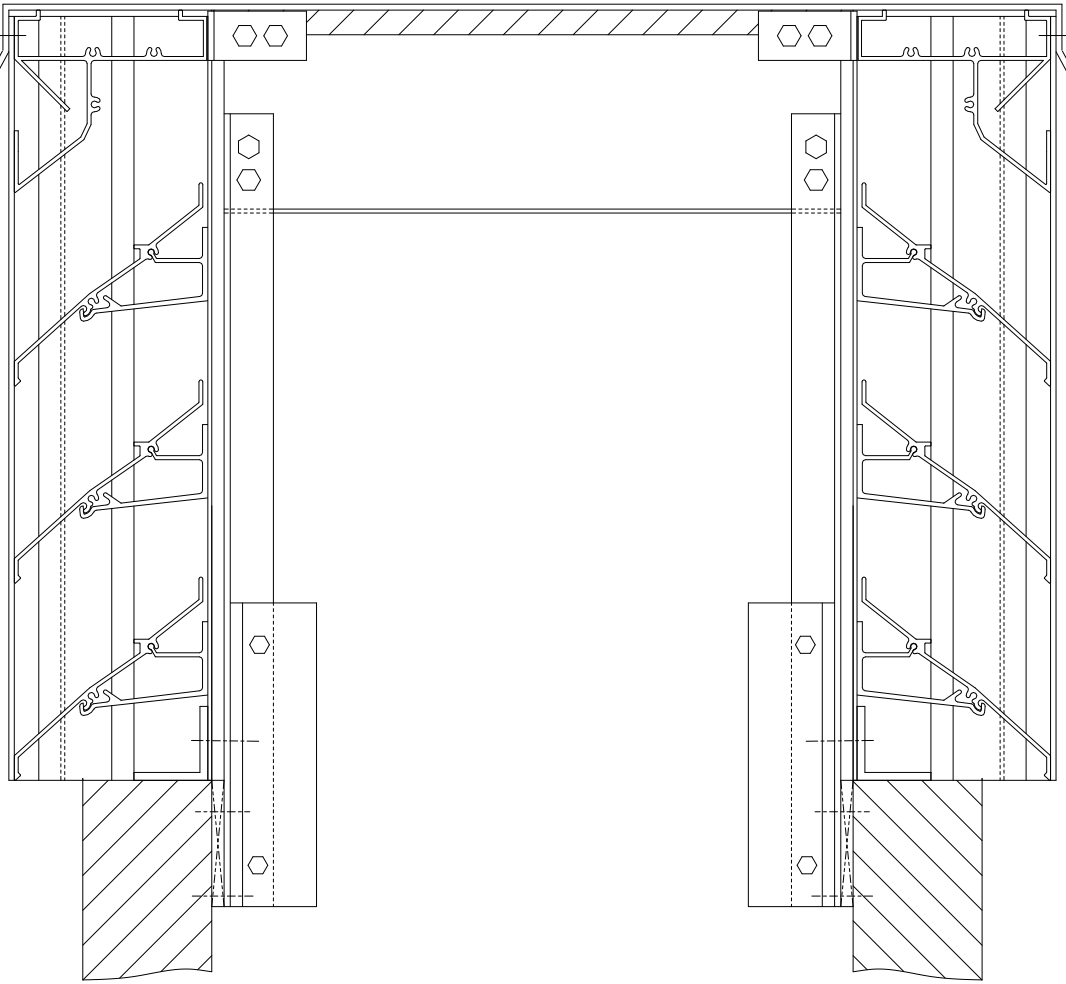
SPH-20-F WITH FLAT ROOF SHOWN
