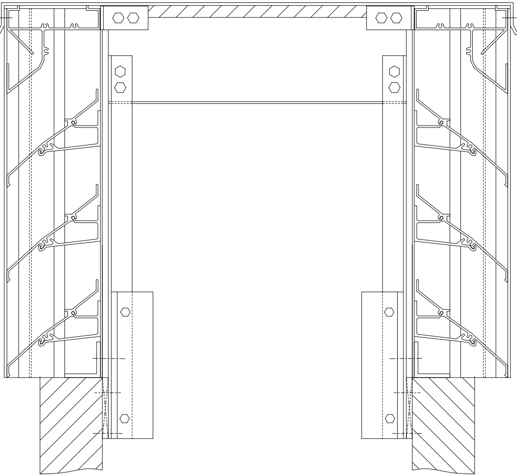
SPH-22-F WITH FLAT ROOF SHOWN
