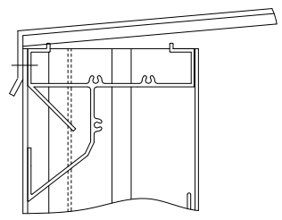
SLOPED ROOF DETAIL
