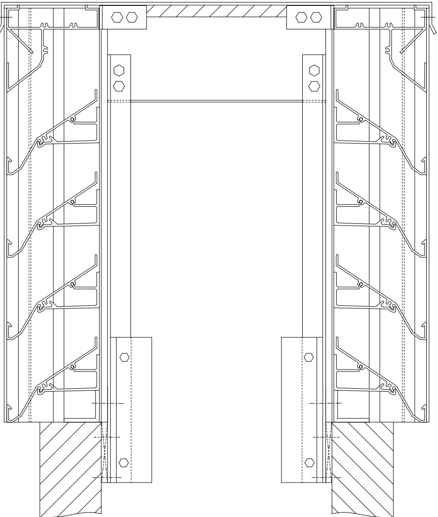
SPH-35-F WITH FLAT ROOF SHOWN
