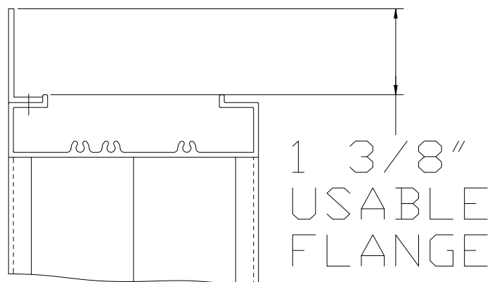
FLANGE FRAME DETAIL
