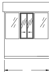
ELEVATION C
