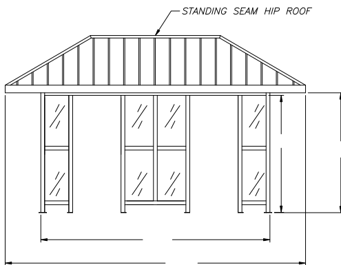
ELEVATION (A)
