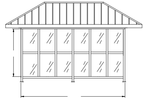
ELEVATION (C)
