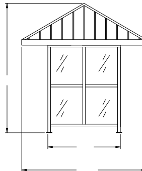
ELEVATION (B&D)
