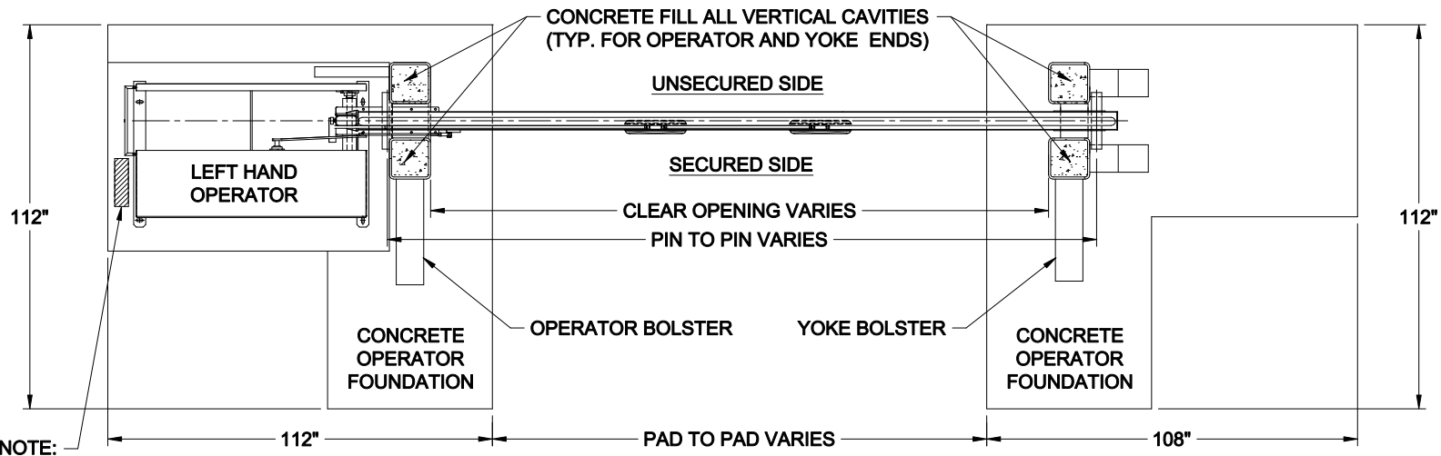
PLAN VIEW
