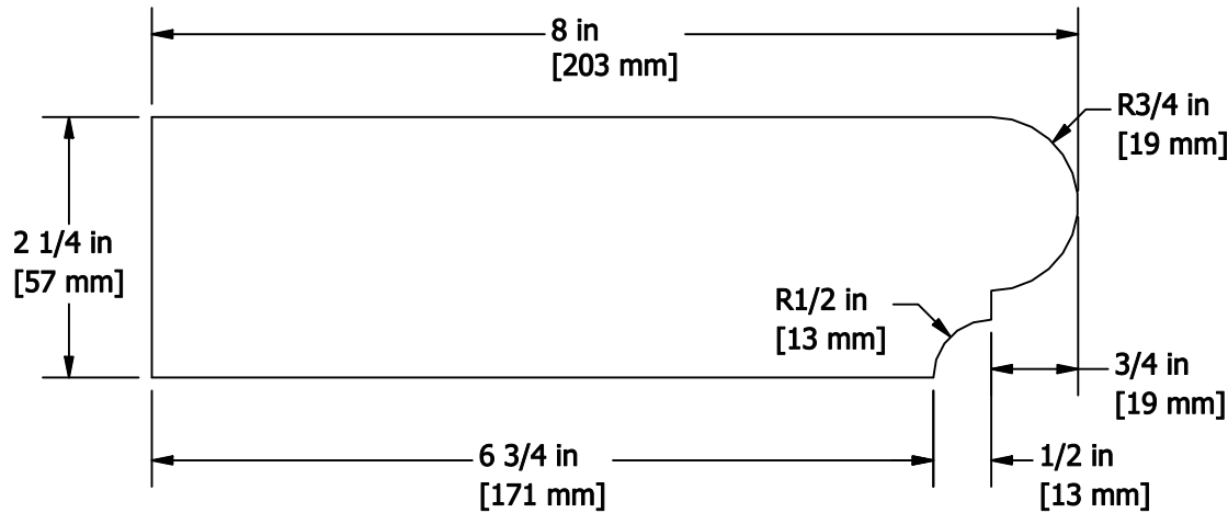
LEFT-SIDE VIEW
