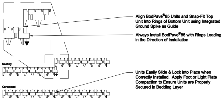
2 BodPave®85 : Snap-Fit Connections Scale : N.T.S.
