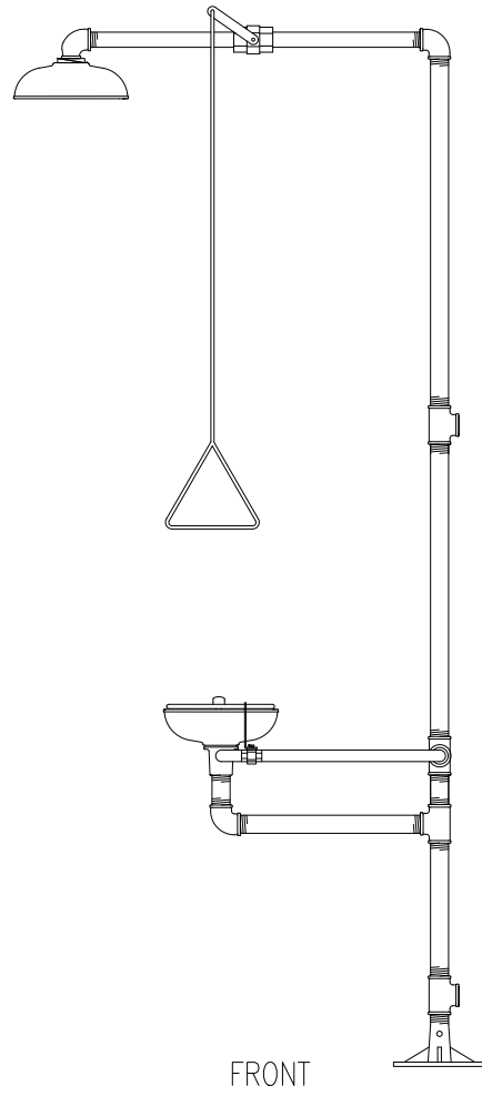
Mod #MS19-310BF Eye & Face Wash/Drench Shower Combo - Barrier Free
