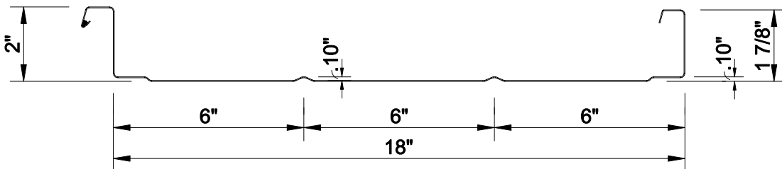
PC 218 Roof Panel With Beaded Pan
