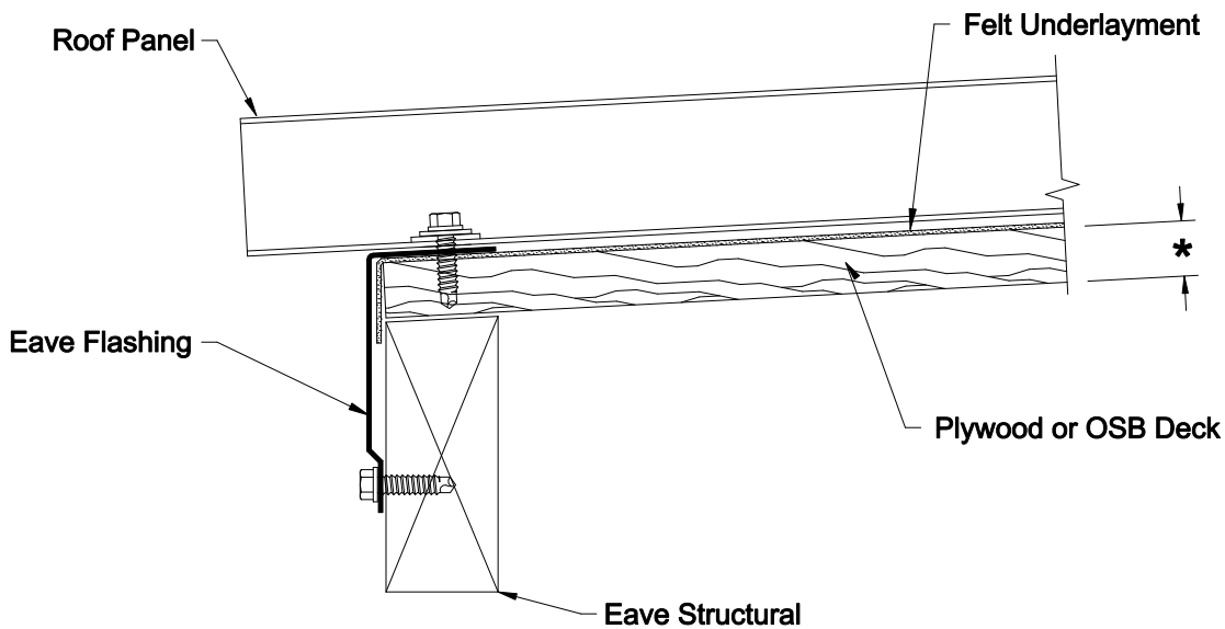
Section @ Eave
