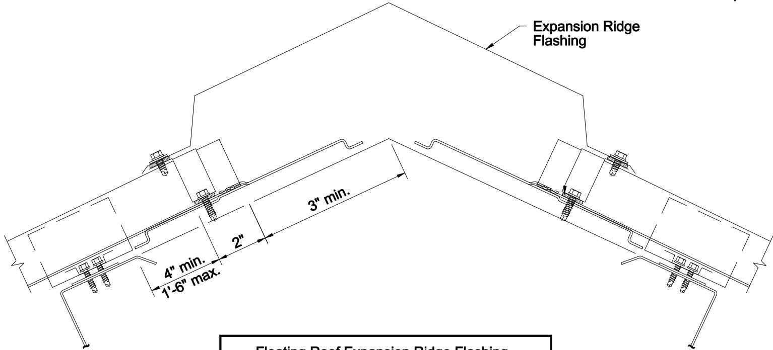
Floating Roof Expansion Ridge Flashing (Accommodates Roof Panel Expansion Movements Required When Roof Run Exceeds 50')
