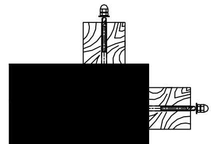
BOTH FITTINGS ATTACH THROUGH POST
