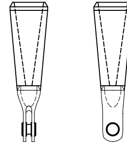
ART-10.750 + UPC-6.625L ART-273 + UPC-168L
