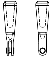
ART-6.625 + UPC-4.000 ART-168 + UPC-102
