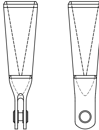
ART-16.000 + UPC-10.750 ART-406 + UPC-273
