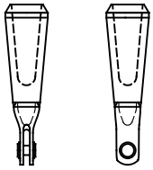
ART-6.625 + UPC-4.000L ART-168 + UPC-102L
