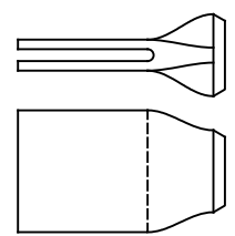
HSC-10.750 HSC-273
