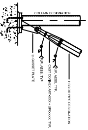
2 BRACE DETAIL
