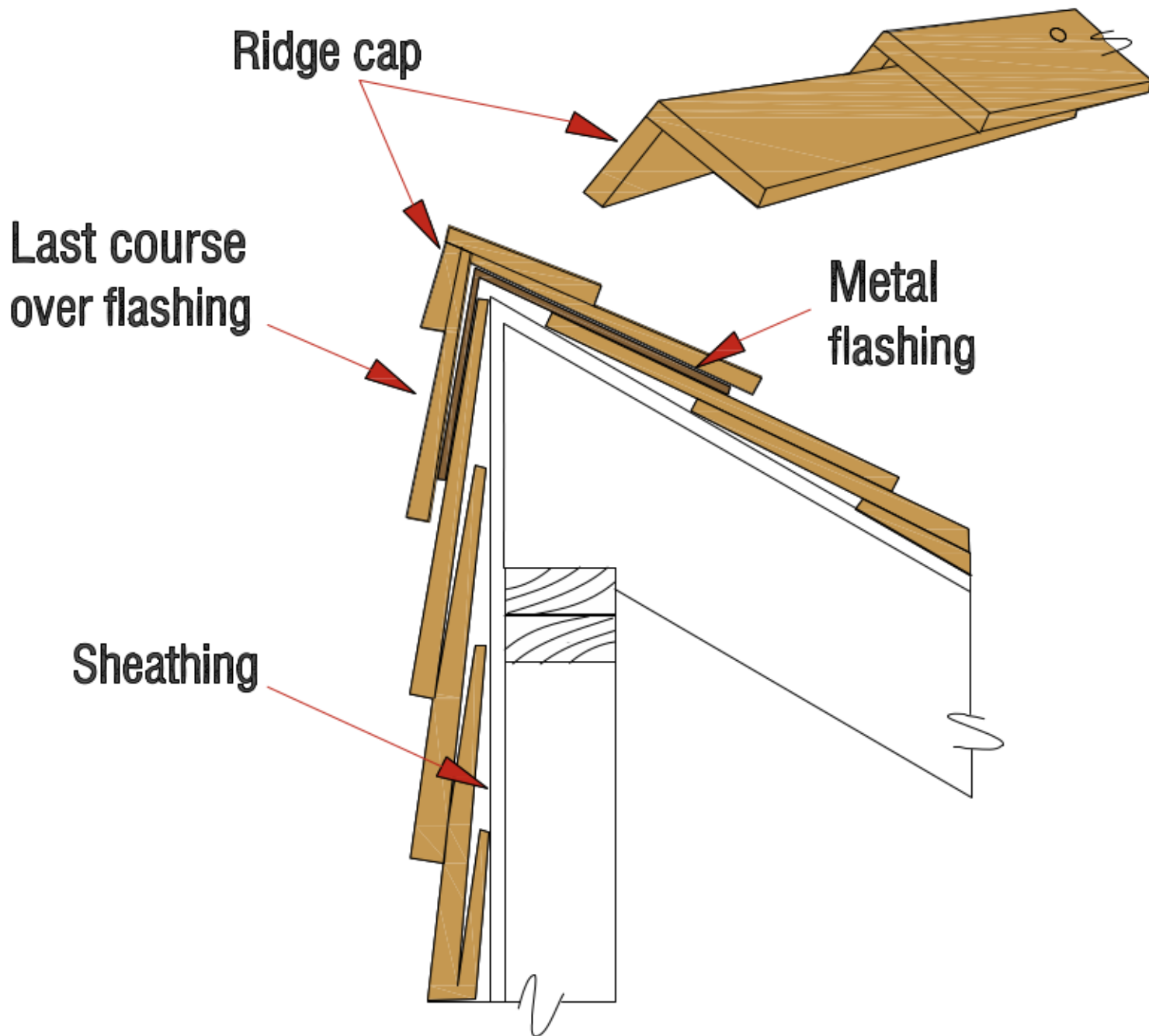
Figure 11: Apex Roof Juncture
