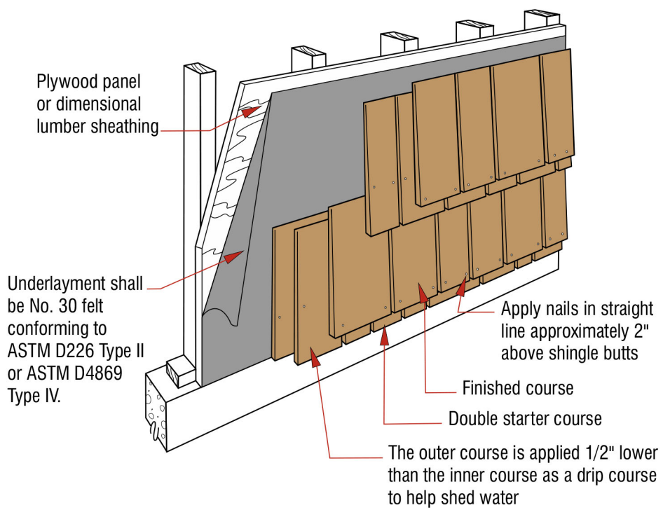
Figure 11: Ribbon Coursing
