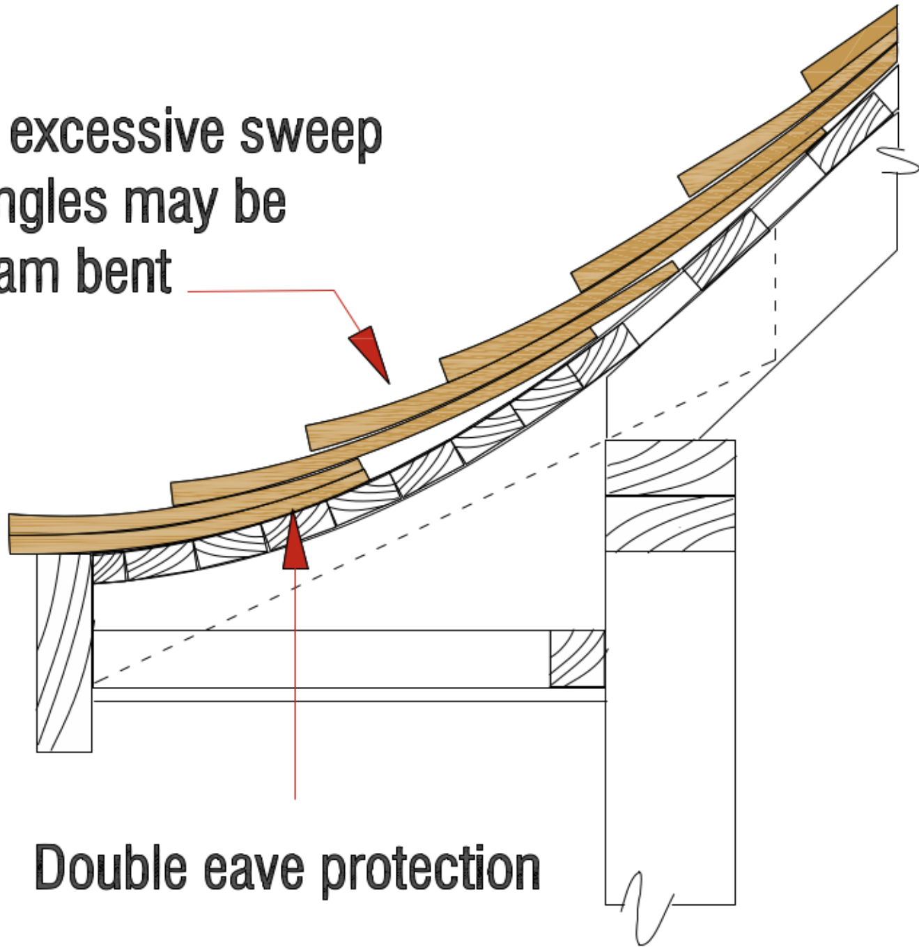
Figure 12: Swept or Bell Eave
