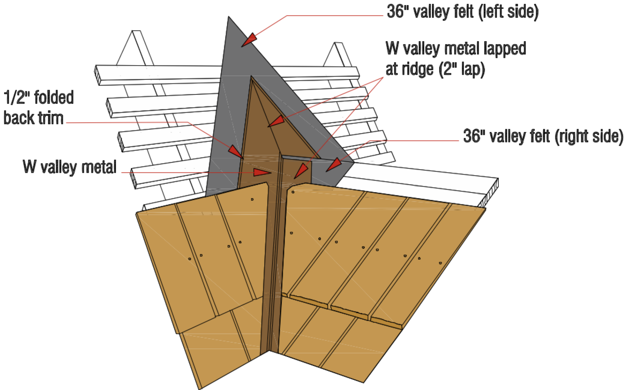
Figure 13b: Typical Saddle Flashing Detail
