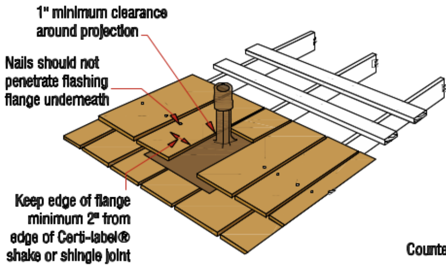
Figure 14d: Typical Projection Flashing
