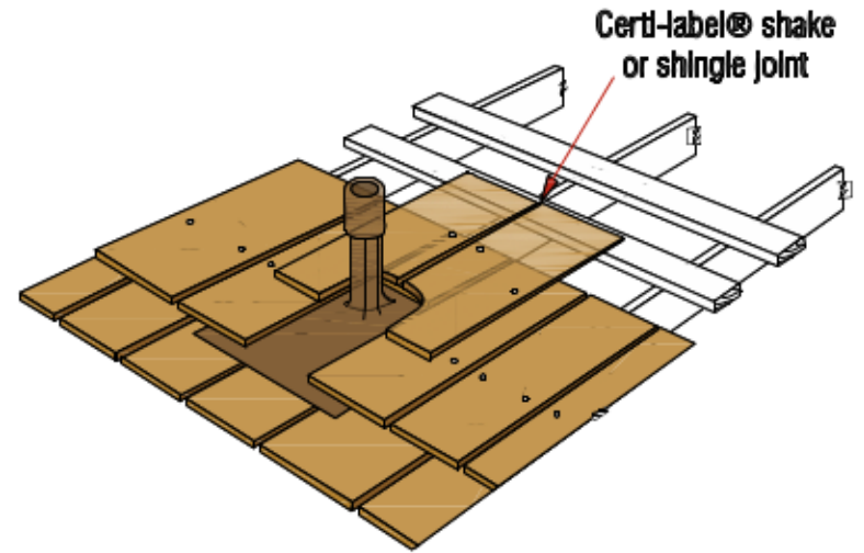
Figure 14e: Typical Projection Flashing
