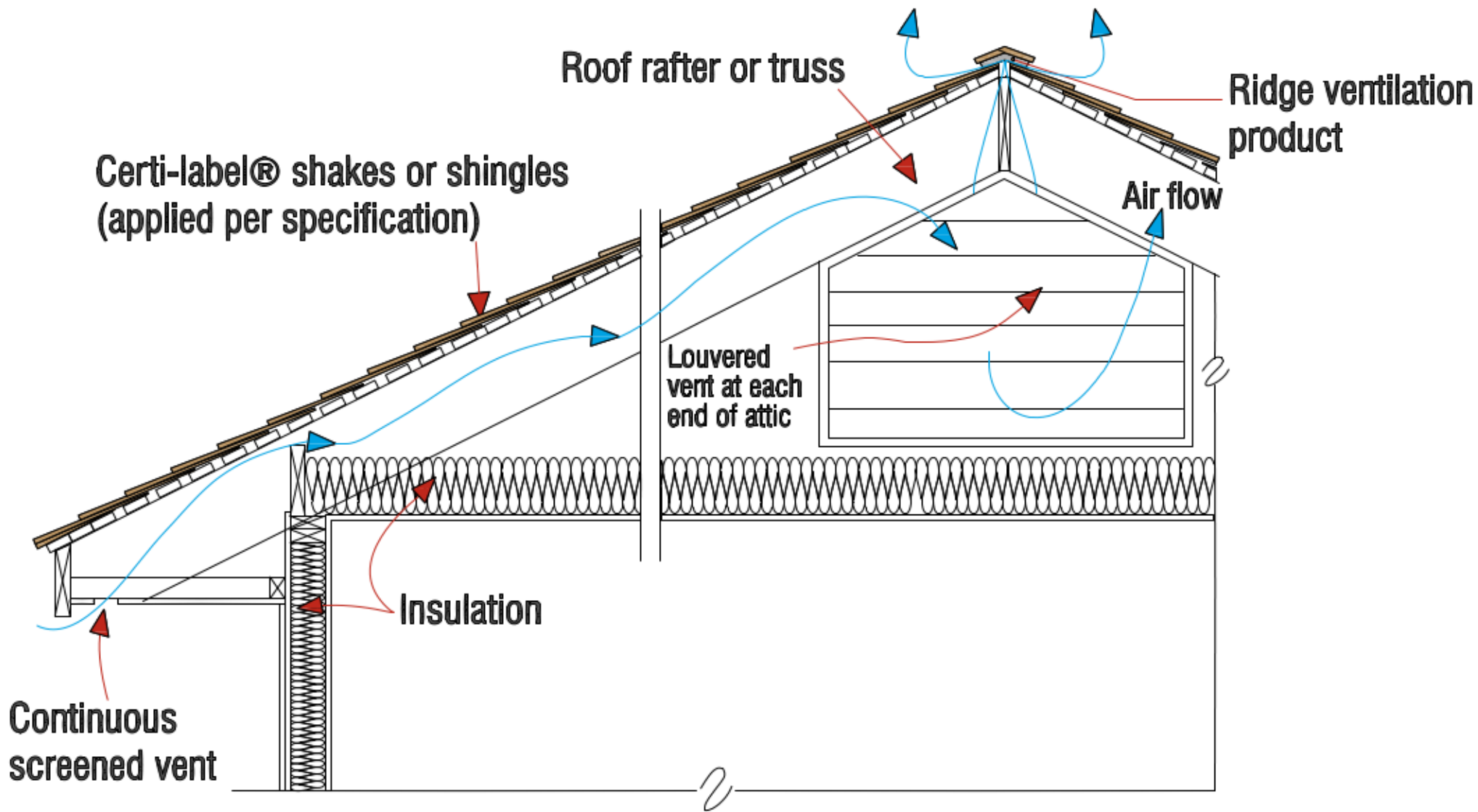
Figure 15a: Gable Roof With Attic
