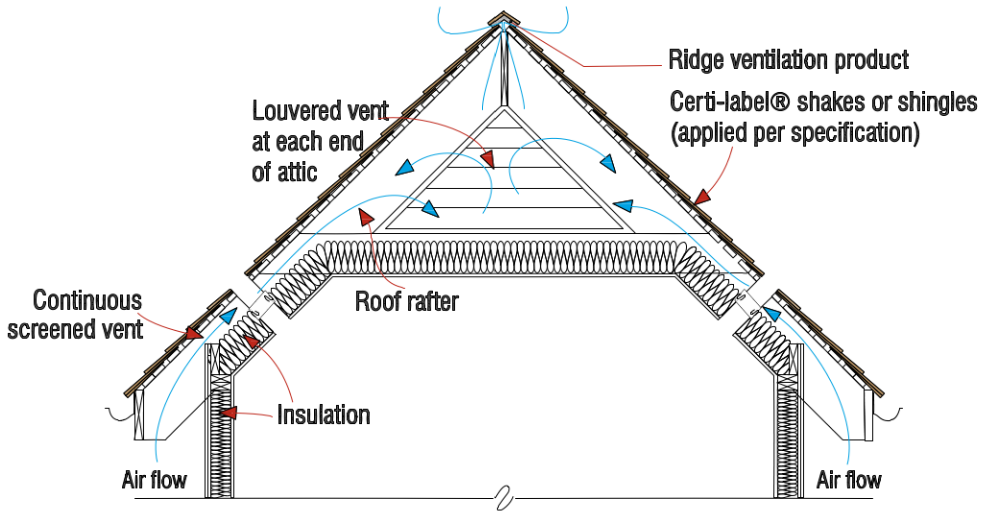
Figure 15b: Cathedral Ceiling With Partial Attic
