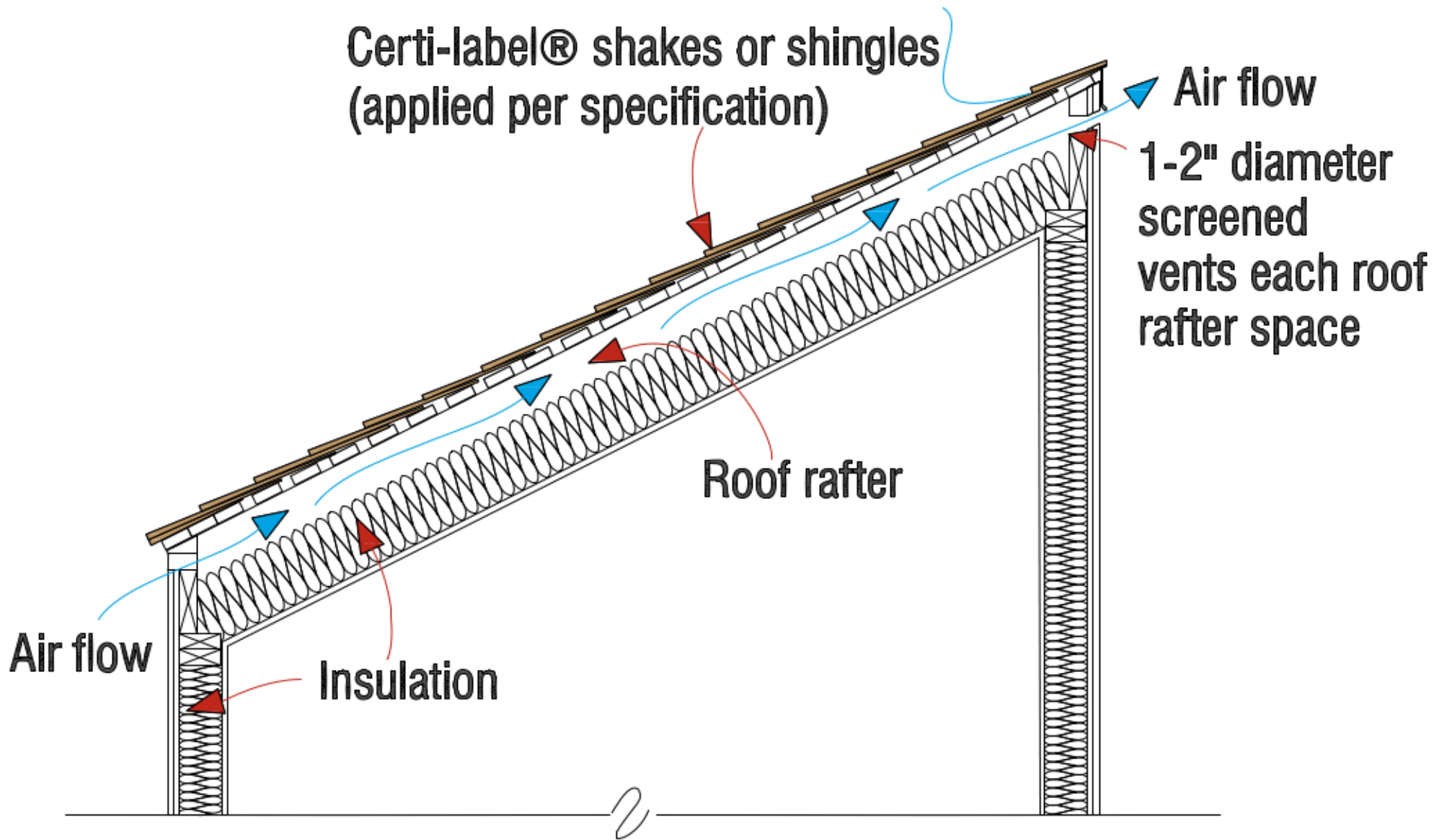
Figure 15c: Shed Roof
