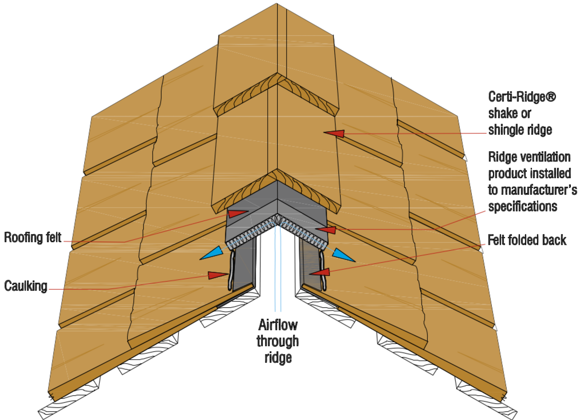
Figure 16: Ridge Ventilation Detail
