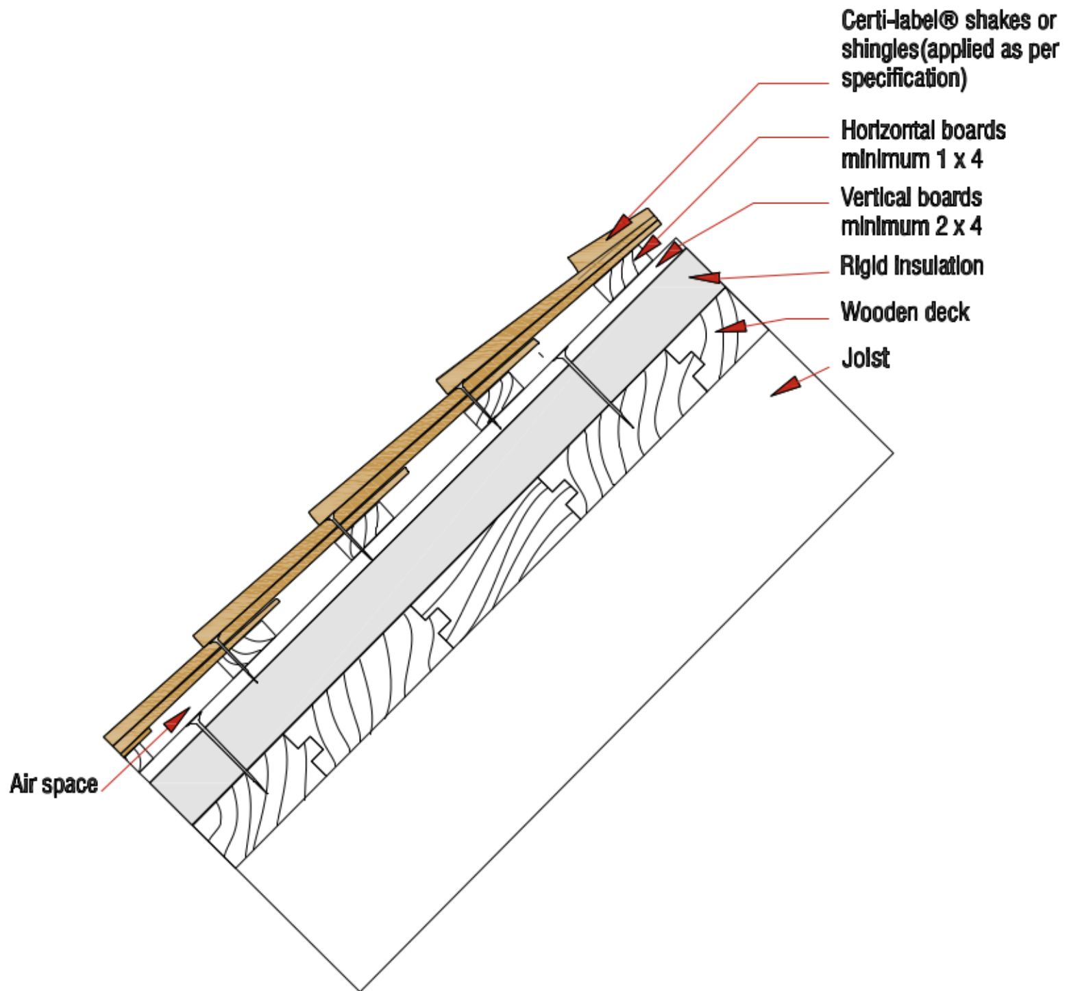
Figure 17: Specialty Roof Deck-Vented Roof
