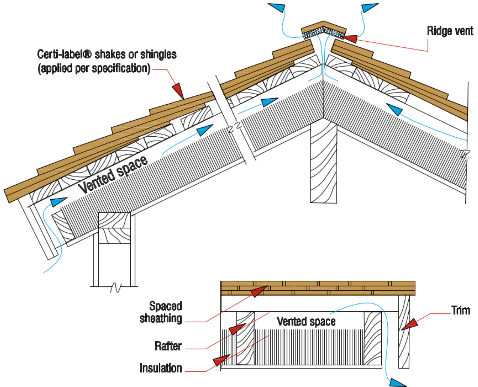
Figure 18: Gable Roof
