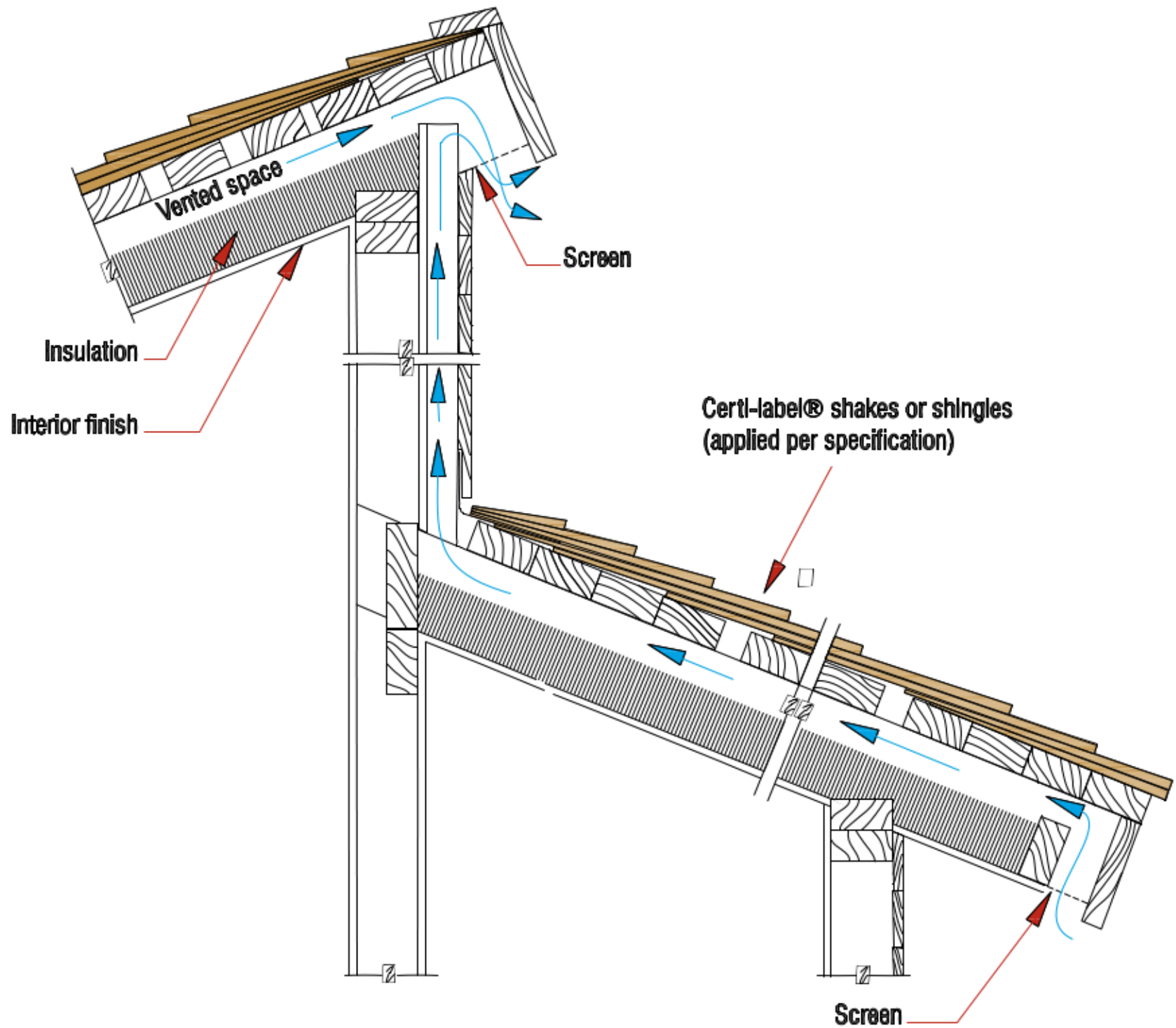
Figure 20: Half Monitor Roof
