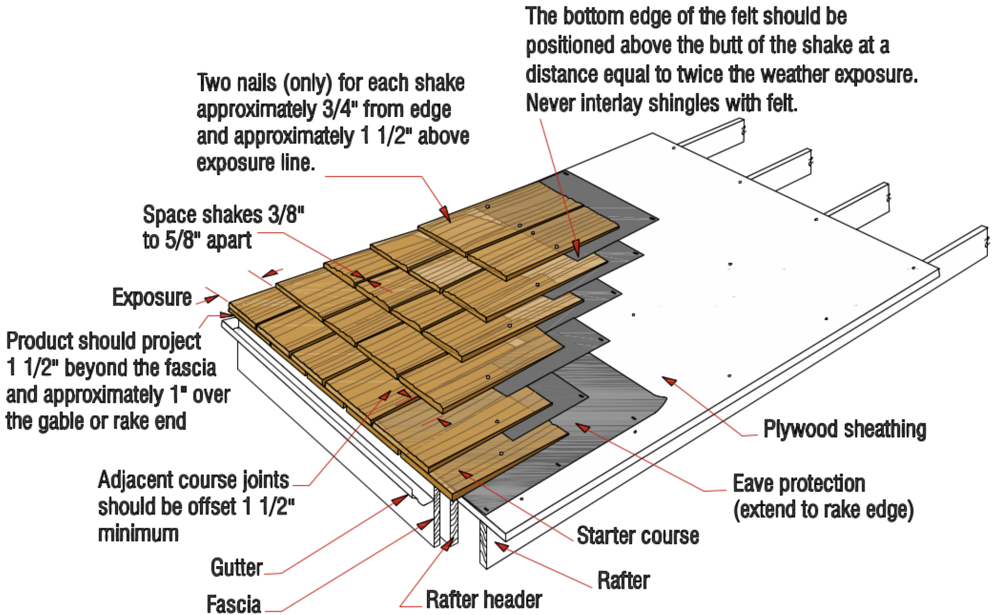
Figure 21a: Certi-Last® Shake Application (Option 1 Depicted)
