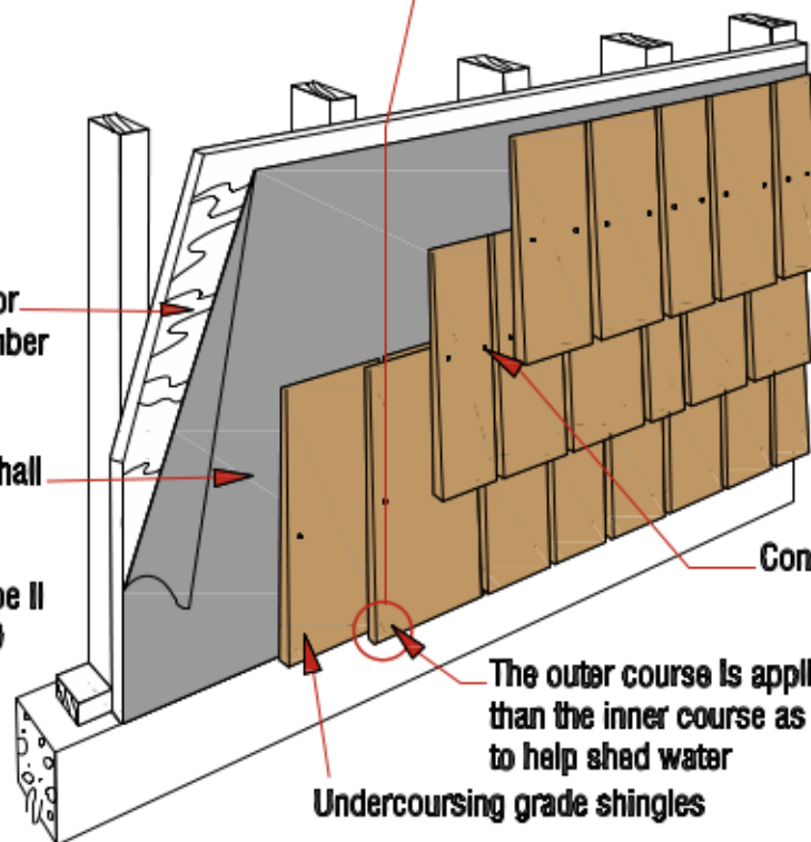
Figure 6: Single Coursing
