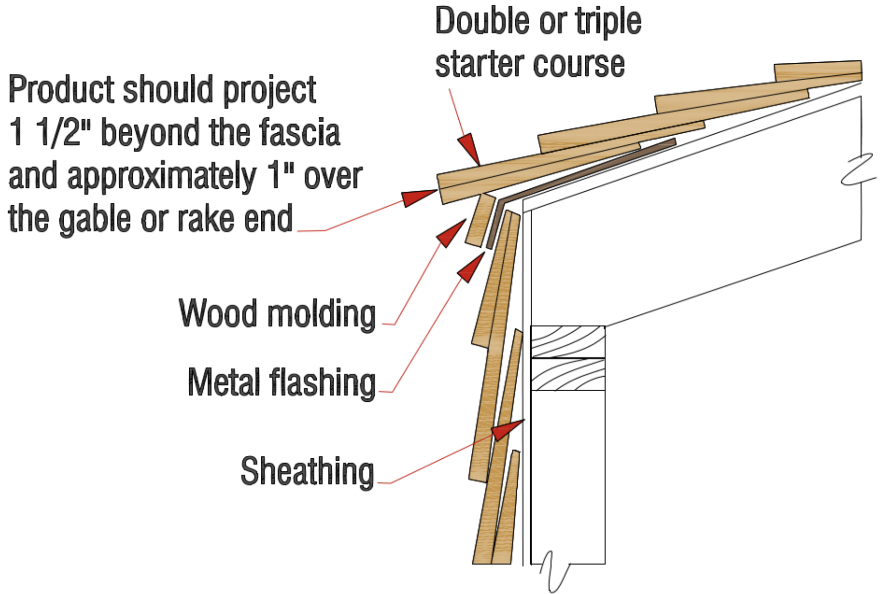
Figure 9: Convex Roof Juncture
