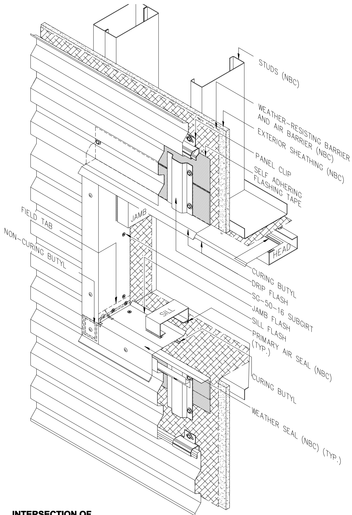
INTERSECTION OF HEAD, JAMB & SILL FLASH (CS-6016)
