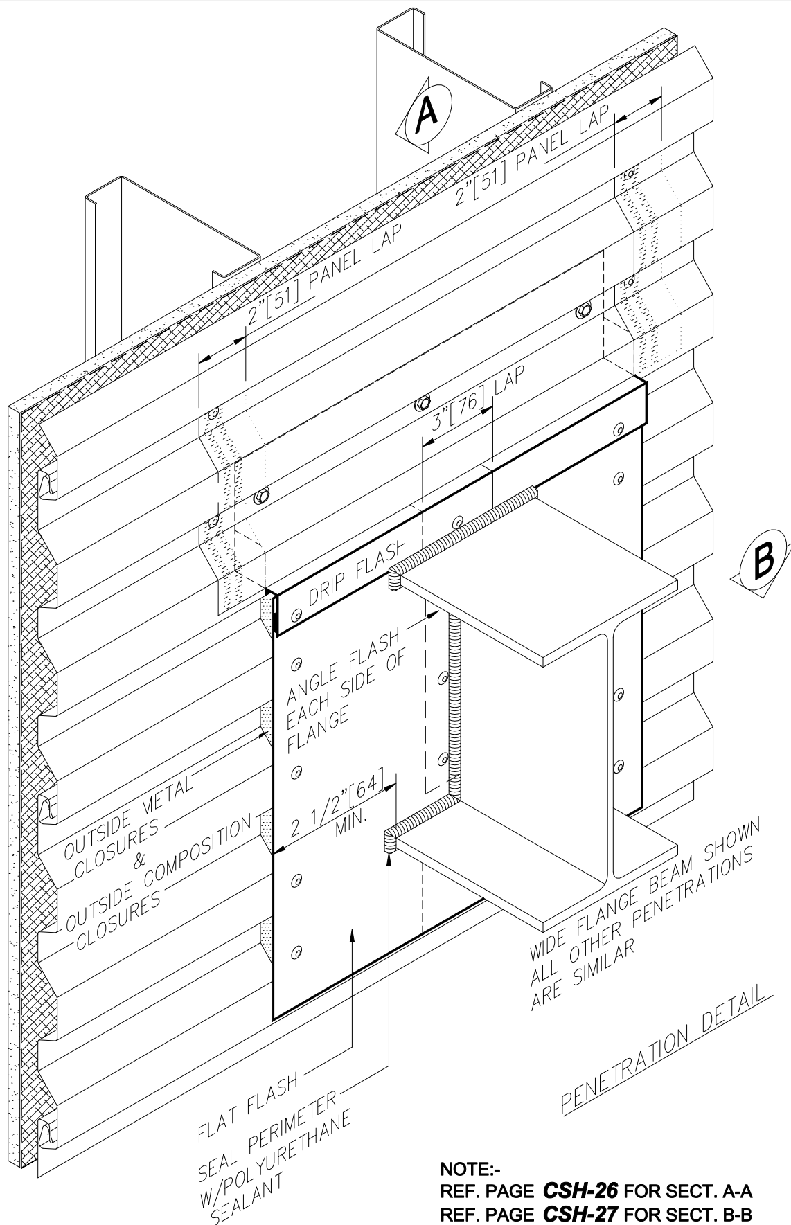
PENETRATION DETAIL (CS-6015)
