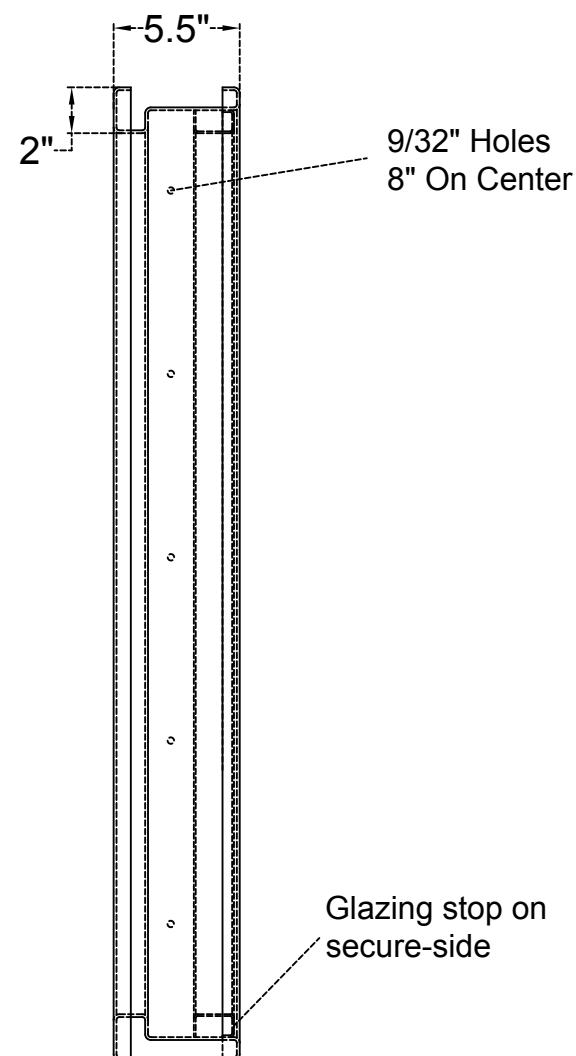
END VIEW
