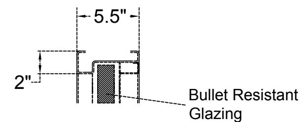
HEAD/JAMB/SILL SECTION
