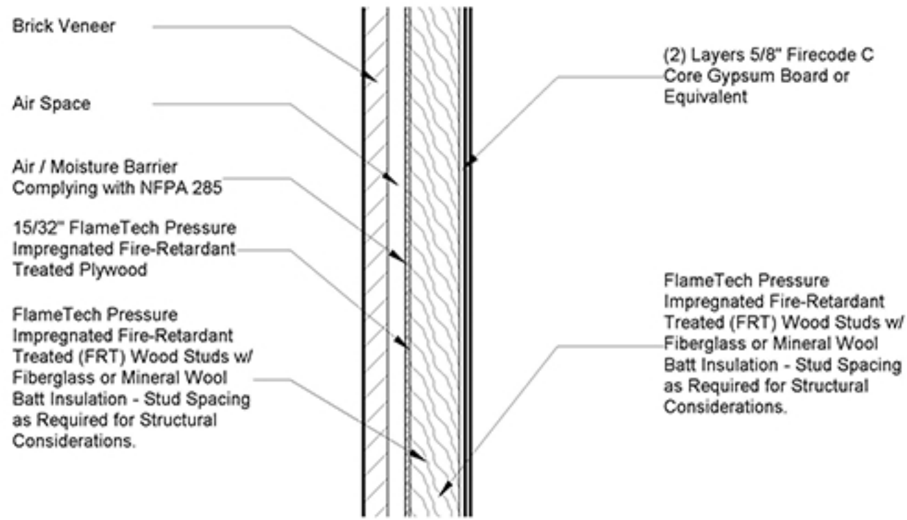
2 FRCT/FRWT 120-02 - Section (Typ.) 3/4" = 1'-0"
