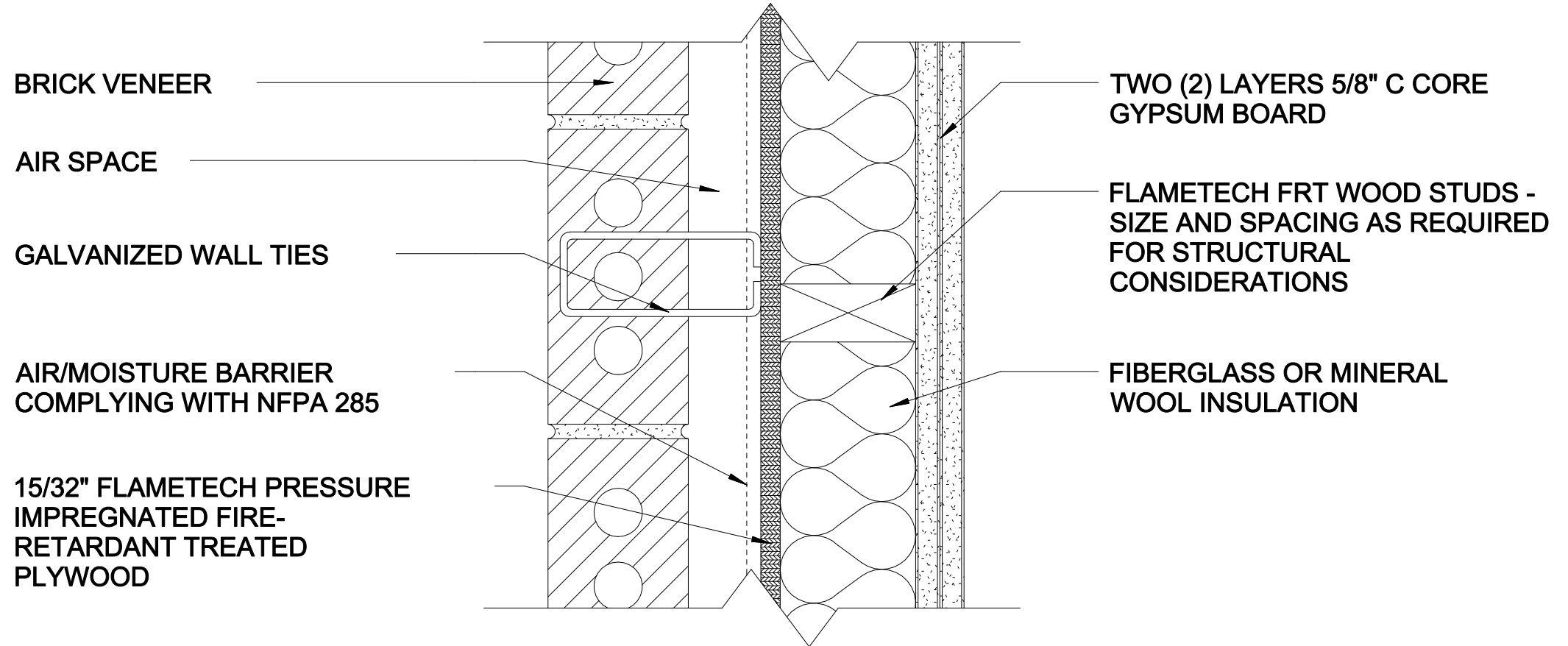
FRCT/FRWT 120-02 BRICK VENEER FINISH ( horizontal cross section )
