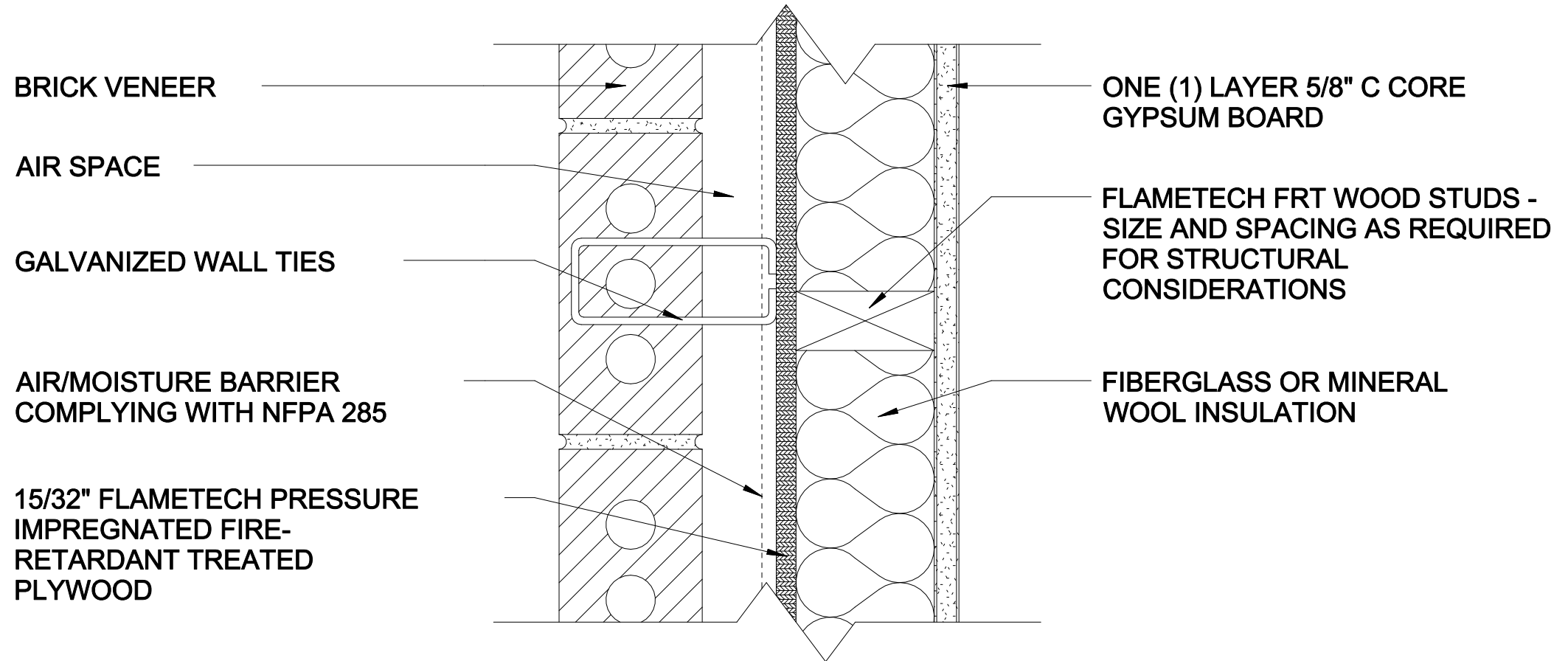
FRCT/FRWT 60-02 BRICK VENEER FINISH ( horizontal cross section )
