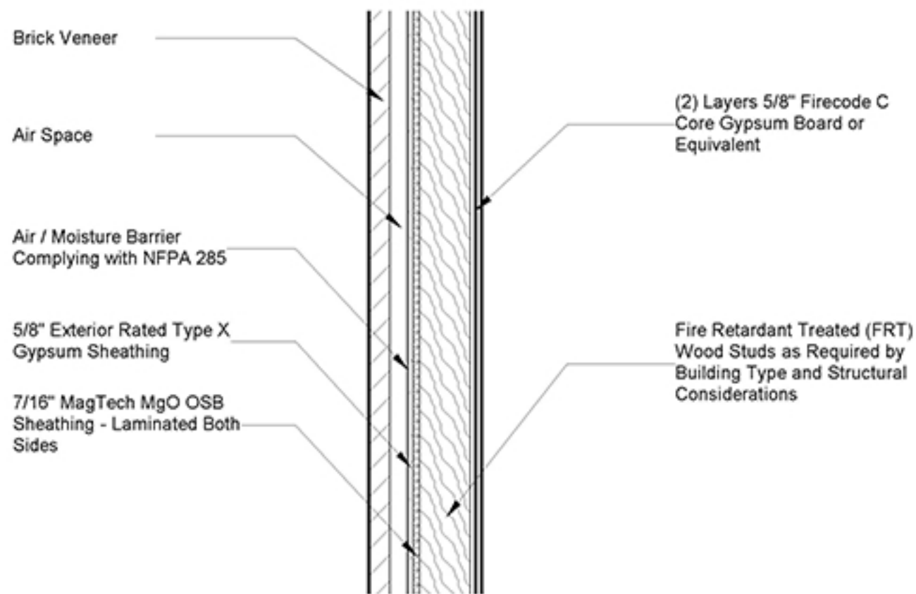
② CF/WPPS 120-03 - Section (Typ.) 3/4" = 1'-0"
