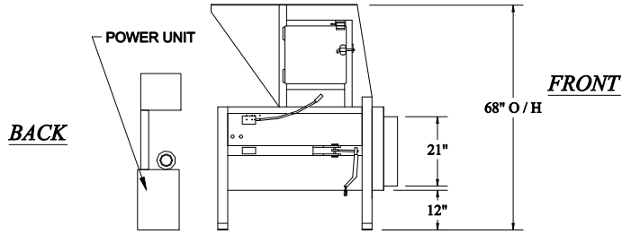
LEFT VIEW
